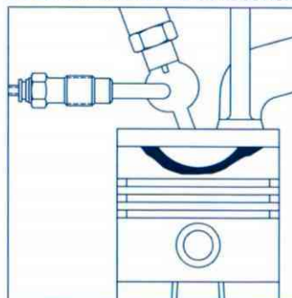
PRE-COMBUSTION
