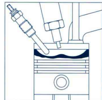
DIRECT INJECTION
